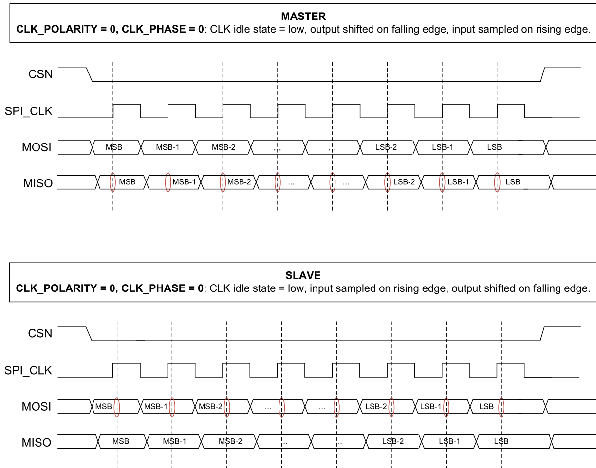
Figure 59. SPI Timing, CLK_POLARITY = 0, CLK_PHASE = 0
