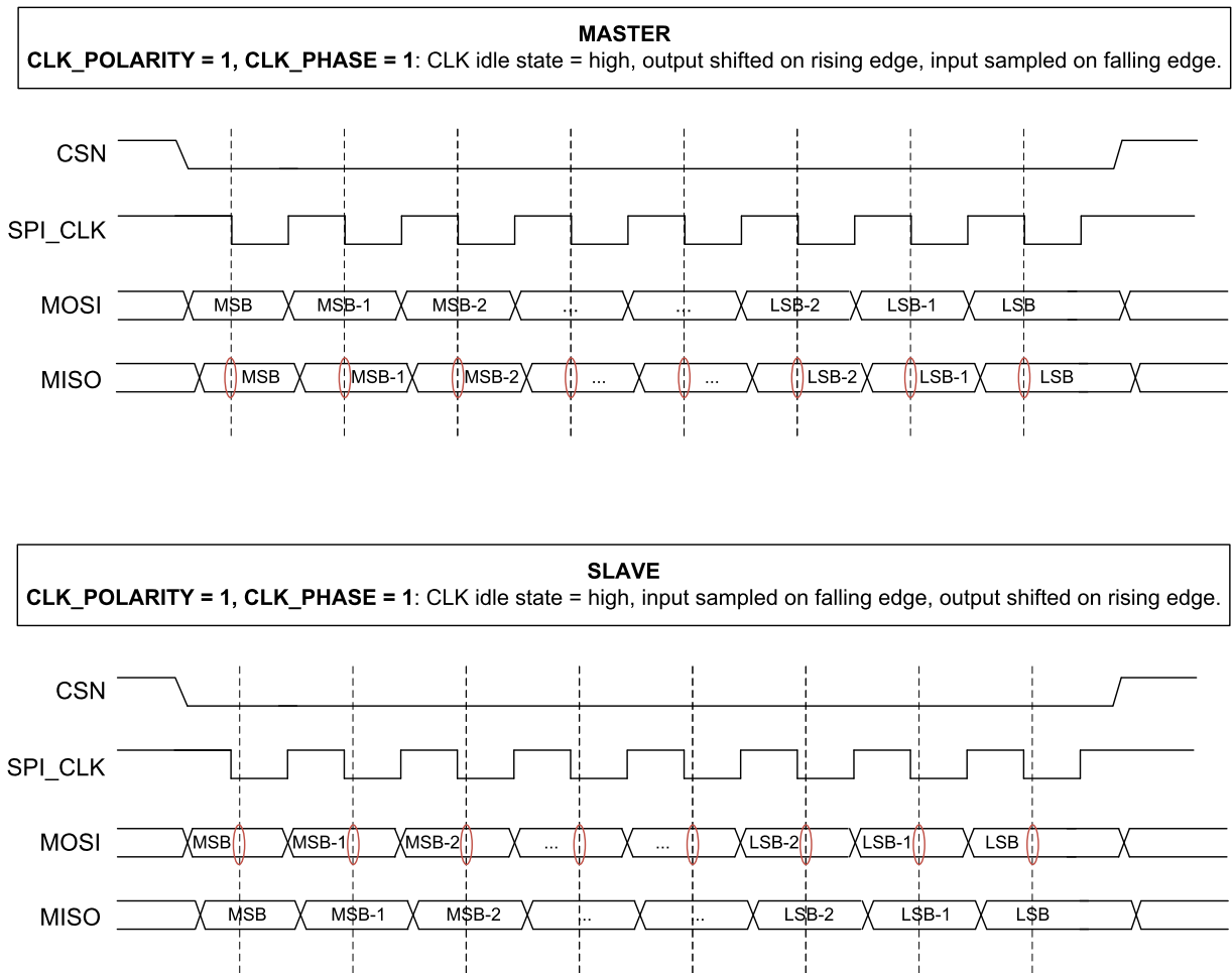
Figure 62. SPI Timing, CLK_POLARITY = 1, CLK_PHASE = 1
