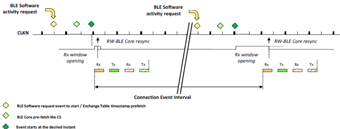
Figure 23. Connection Event Programming and Exchange Table Pre-Fetch / Slave Device Example
