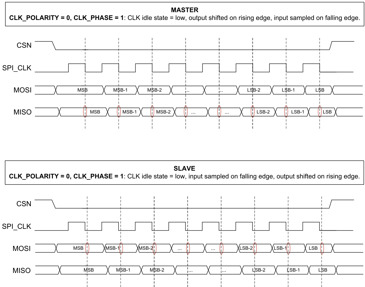
Figure 60. SPI Timing, CLK_POLARITY = 0, CLK_PHASE = 1
