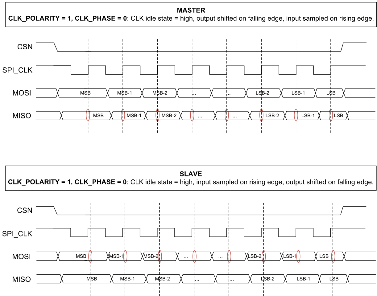
Figure 61. SPI Timing, CLK_POLARITY = 1, CLK_PHASE = 0
